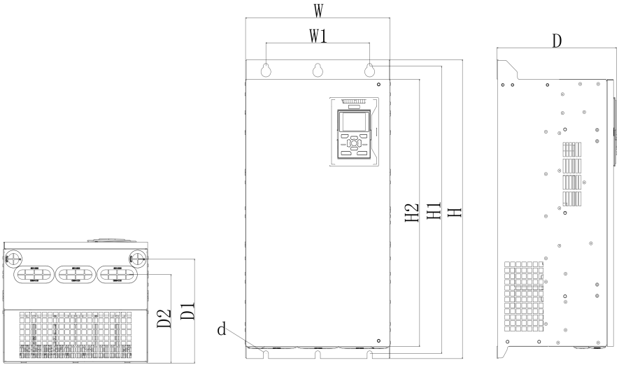
(c) 030G/037P~400G/450P 变频器外形
