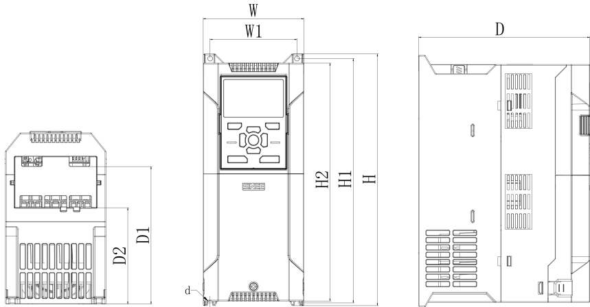
(b) 0R7G/1R5P~022G/030P 变频器外形
