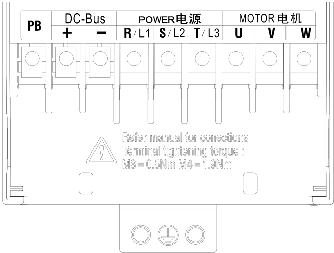
(b) EM750-2R2G/3R0P-3B~EM750-4R0G/5R5P-3B 端子示意图
