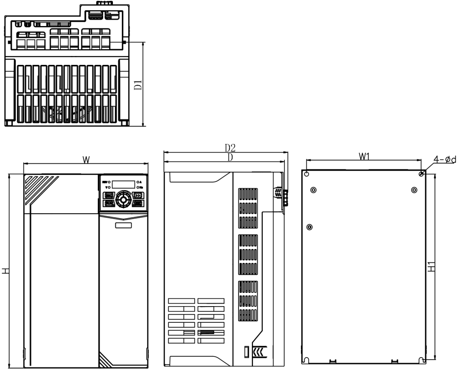
(a) EM750-0R7G/1R5P-3B~EM750-022G/030P-3B 变频器外形
