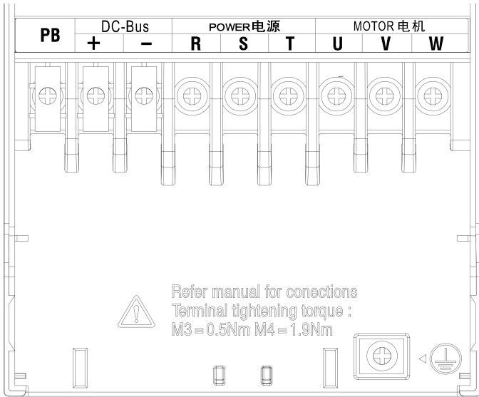
(c) EM750-5R5G/7R5P-3B~EM750-022G/030P-3B 端子示意图, 接地位置略有差异
