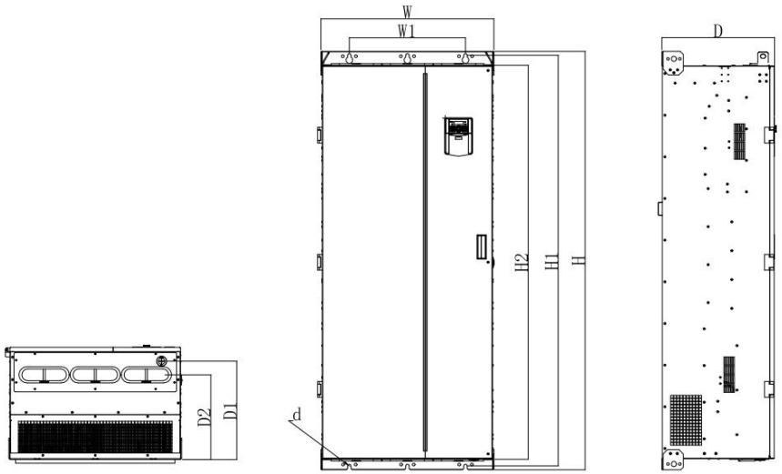
(g) EM750-355G-3~EM750-450G-3 变频器外形
