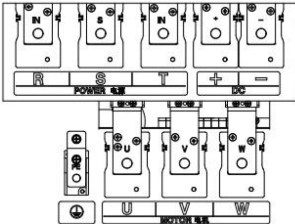
(g) EM750-185G-3~EM750-250G-3 端子示意图
