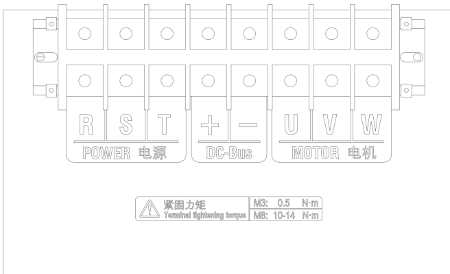
(e) EM750-045G/055P-3~EM750-110G/132P-3 端子示意图
