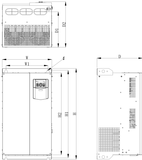
(c) EM750-090G/110P-3~EM750-160G/185P-3 变频器外形
