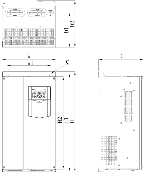
(b) EM750-030G/037P-3B~EM750-075G/090P-3 变频器外形
