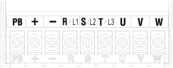
(a) EM750-0R7G/1R5P-3B~EM750-1R5G/2R2P-3B 端子示意图
