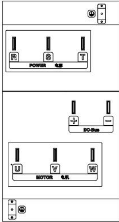
(h) EM750-280G-3~EM750-450G-3 端子示意图
