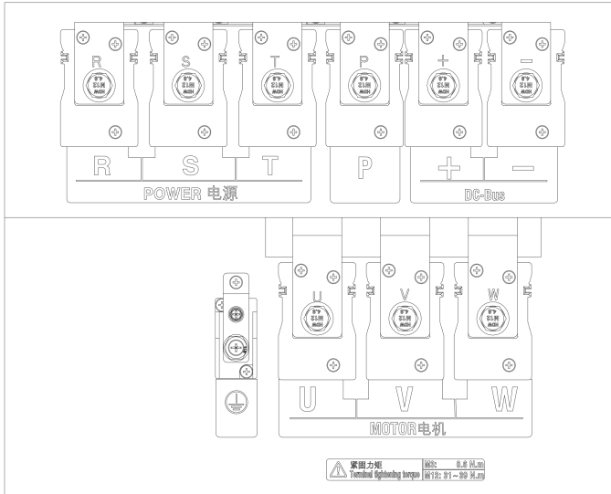
(f) EM750-132G/160P-3~EM750-160G/185P-3 端子示意图
