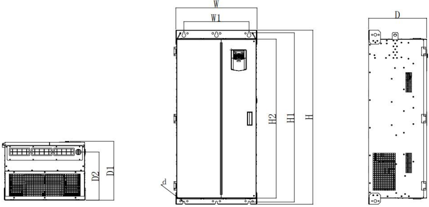
(f) EM750-280G-3~EM750-315G-3 变频器外形
